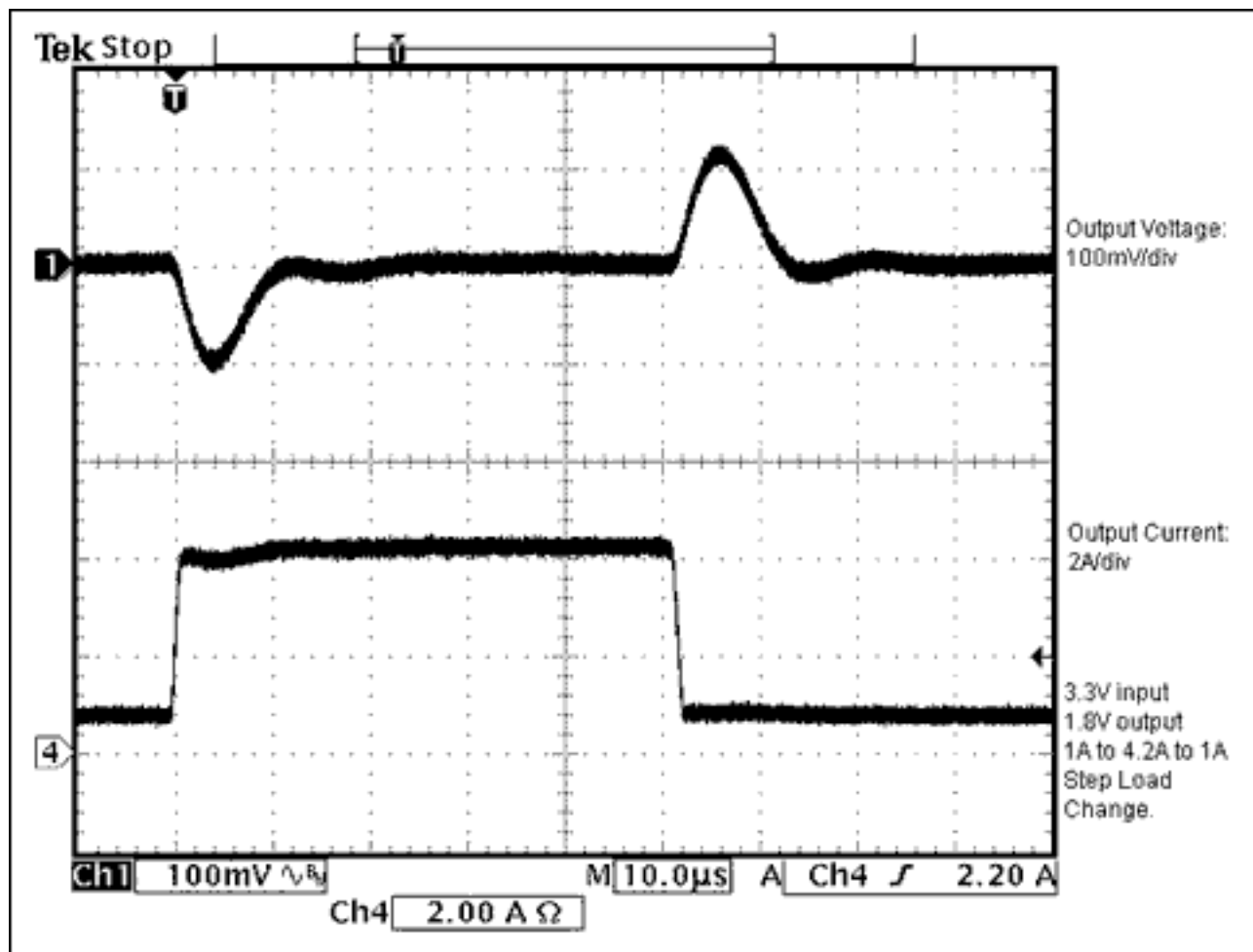
Figure 3. Step load transient response: output current from 1A to 4.2A back to 1A. The output voltage back to regulation within 10 \mu s for 50% step load change.
